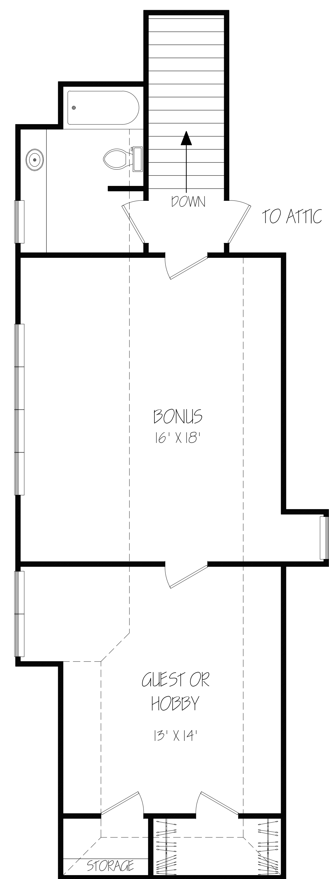
2 SECOND FLOOR 1,004 SQ. FT. (FINISHED)
