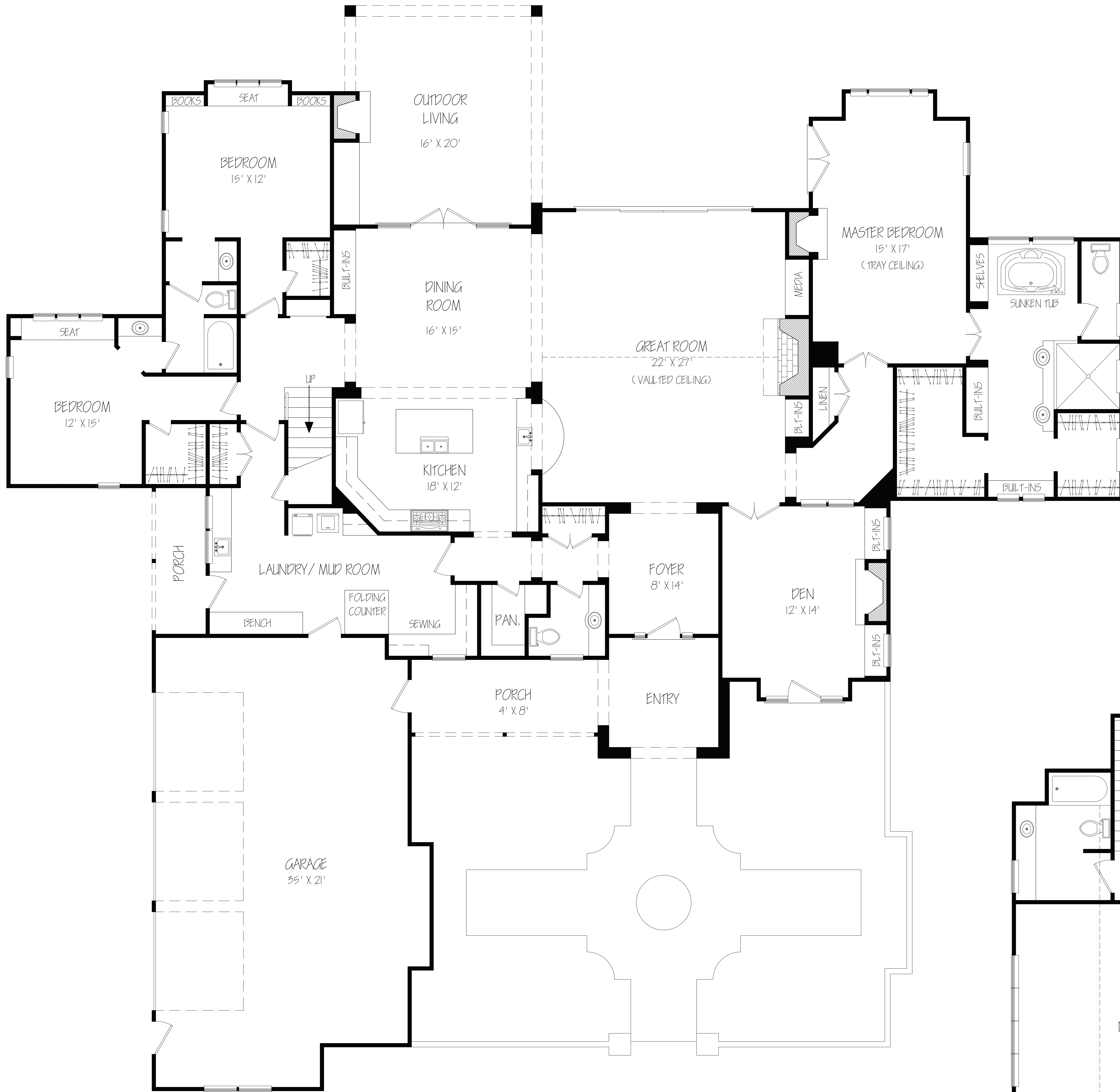
1 FIRST FLOOR 3,711 SQ. FT. (FINISHED) 5,359 SQ. FT. (UNDER ROOF)
